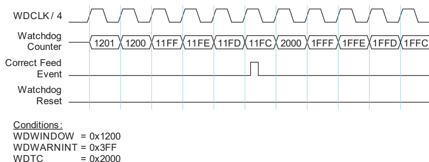
Fig 39. Correct watchdog feed with windowed mode enabled
