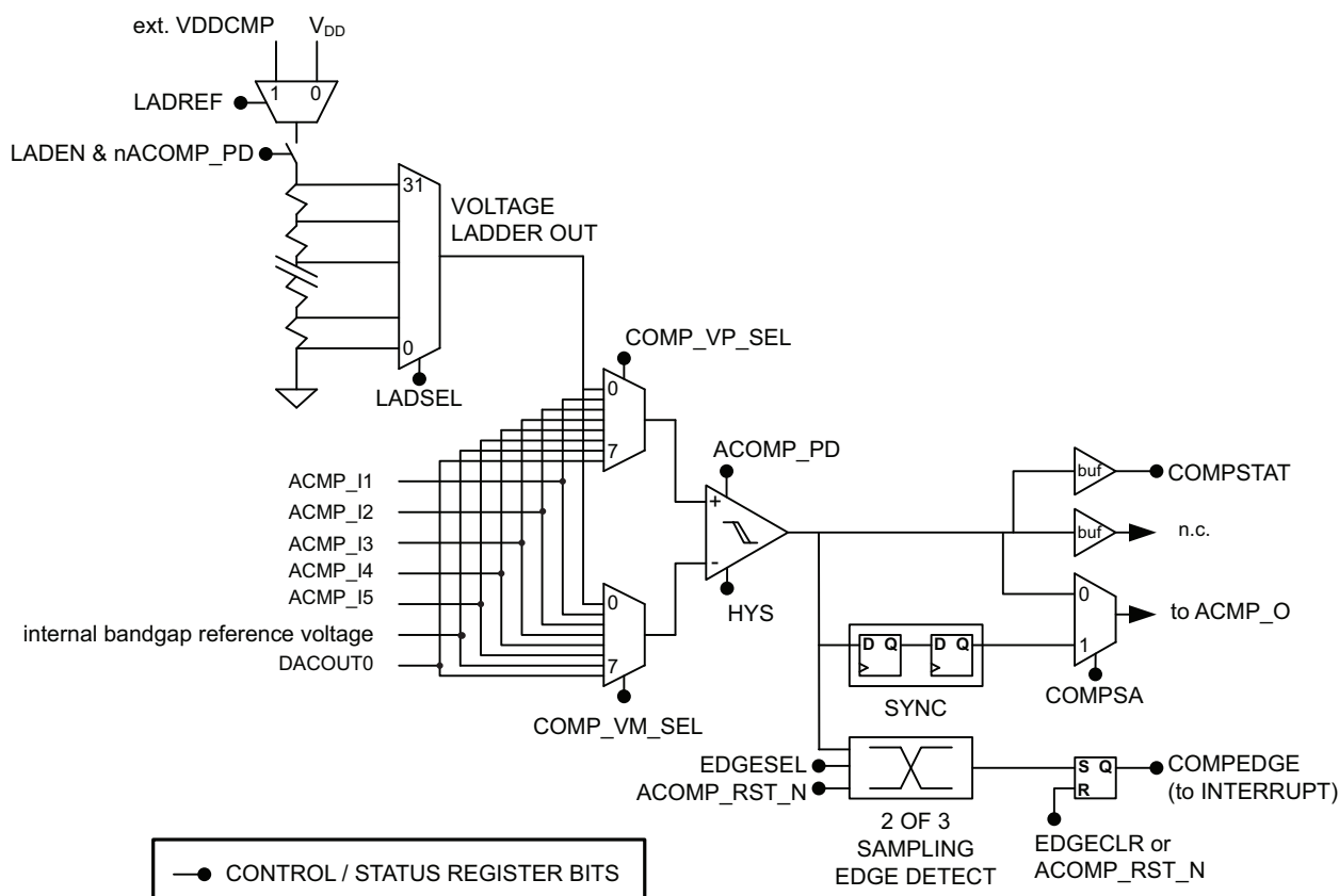
Fig 49. Comparator block diagram
