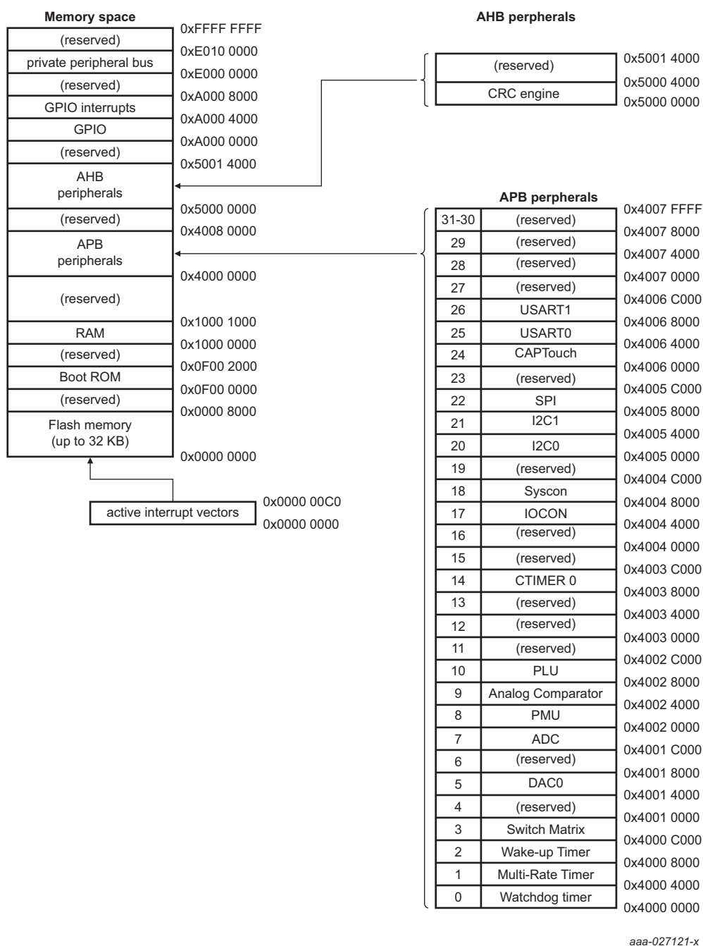
Fig 2. LPC80x Memory mapping <Final>
