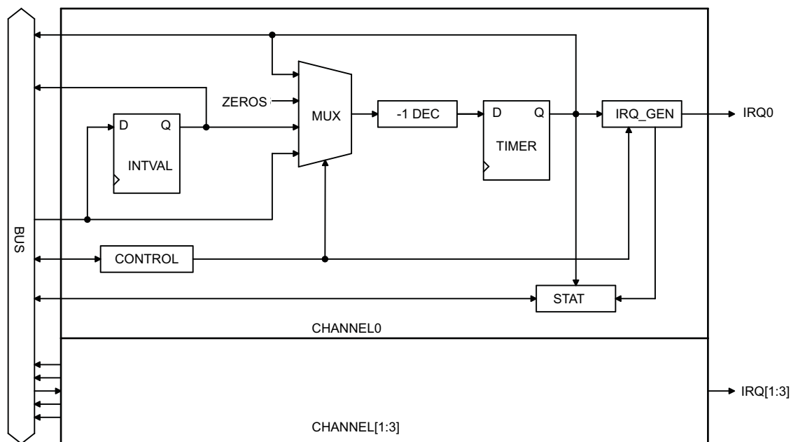
Fig 43. MRT block diagram
