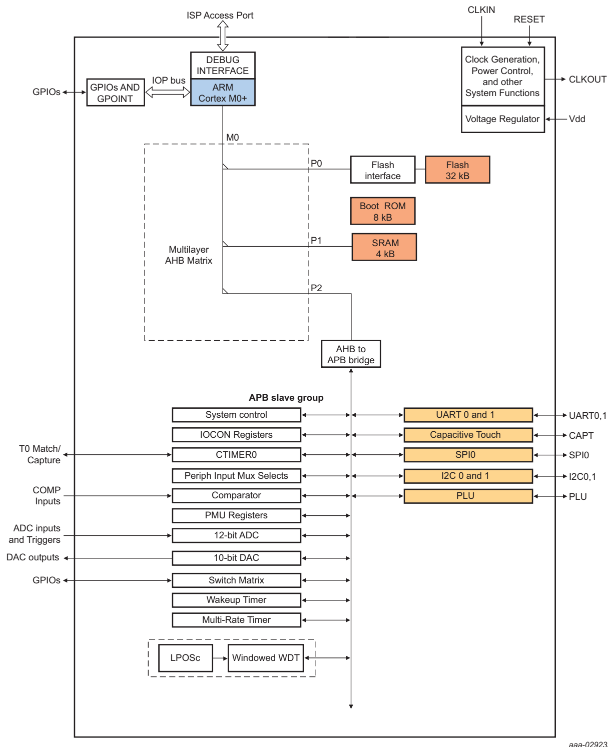
Fig 1. LPC80x block diagram (aaa-029233)
