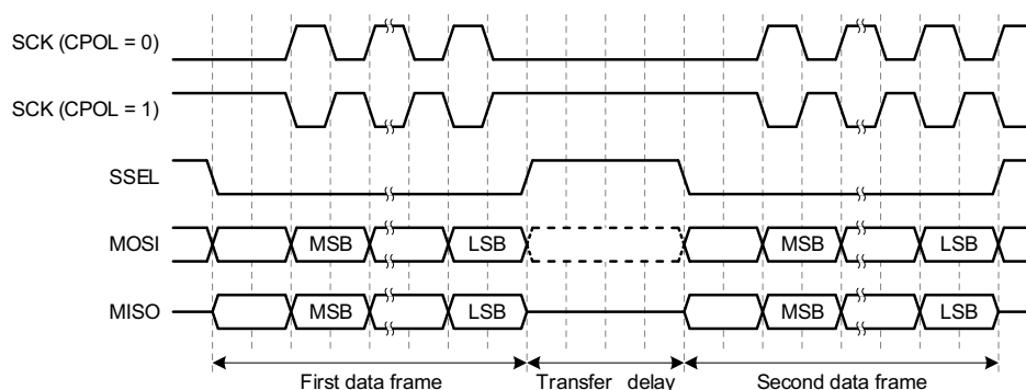
Fig 28. Transfer_delay
